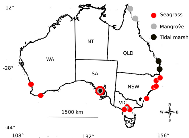
Fig. 1. Locations from individual studies and ecosystems incorporated in the meta-analysis. WA – Western Australia; NT – Northern Territory; SA – South Australia; QLD – Queensland; NSW – New South Wales; VIC – Victoria; TAS – Tasmania (see Table 2 In supplementary materials).
