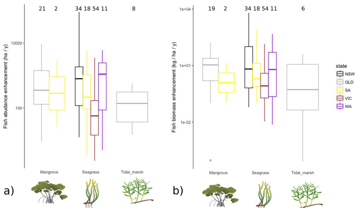
Fig. 2. Boxplot of fish-specific (a) abundance (ha -1 y -1 ) and (b) biomass (kg ha -1 y -1 ) enhancement from mangrove, seagrass and tidal marsh ecosystems compared to unvegetated seabed across five Australian states. Numbers above each box show the number of individual fish species enhanced by coastal ecosystems for each state. See Fig. 1 for state abbreviations.
